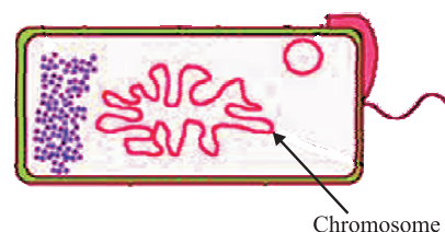
Fig. 25.3a Bacterial chromosome
