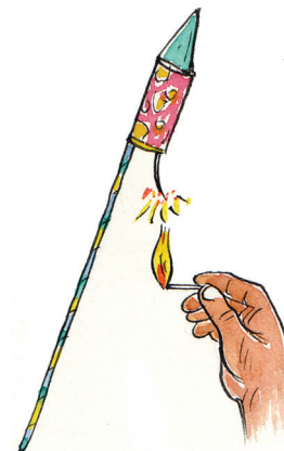
(b) Bursting of fireworks (chemical energy → heat, light and sound energy)
